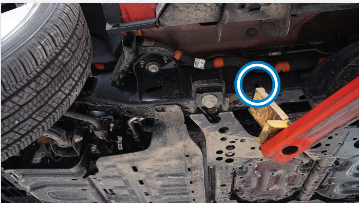
Driver side front frame rail jacking location
