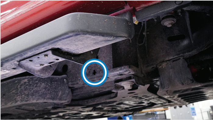
Passenger side front frame rail jacking location
